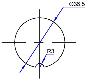
Tank hole dimensions
